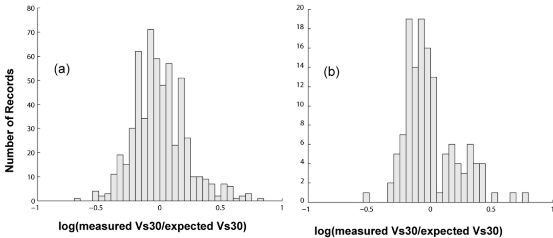
Figure 7: Histograms indicating logarithmic differences of measured V_{s,30} values compared to the expected V_{s,30} assuming a lognormal distribution ( 426\text{m/s} for active regions (a) and 424\text{m/s} for stable regions (b)). The biases are null as expected and the standard deviations are 0.219 for active and 0.214 for stable regions.
